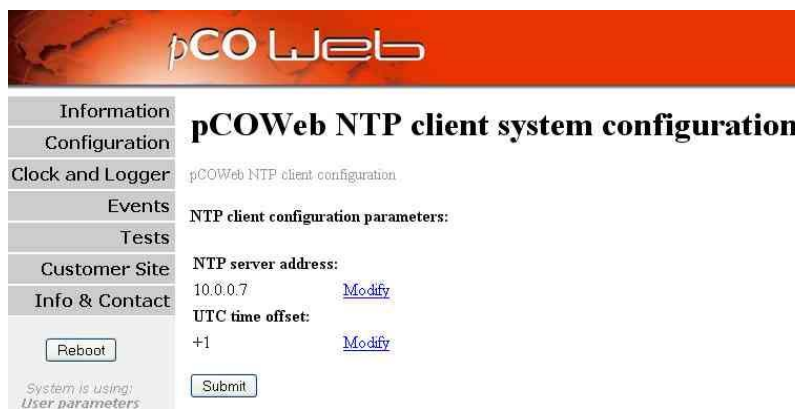
Figure 9.s – Page for setting the “NTP” Plugin parameters
