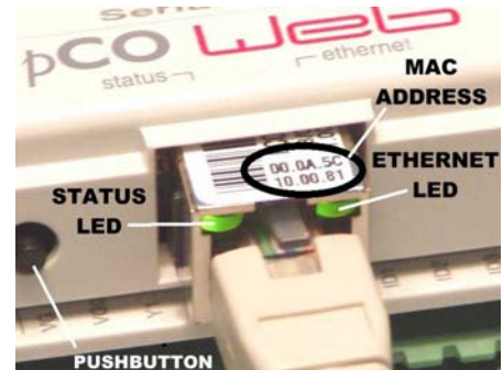
Figure 1.b - MAC address and indicator LEDs
